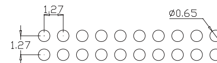
Recommended PCB Layout (PCB TOLERANCE \pm 0.05 )
